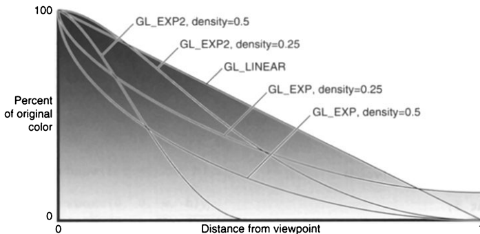
Figure 6-4 Fog-Density Equations
