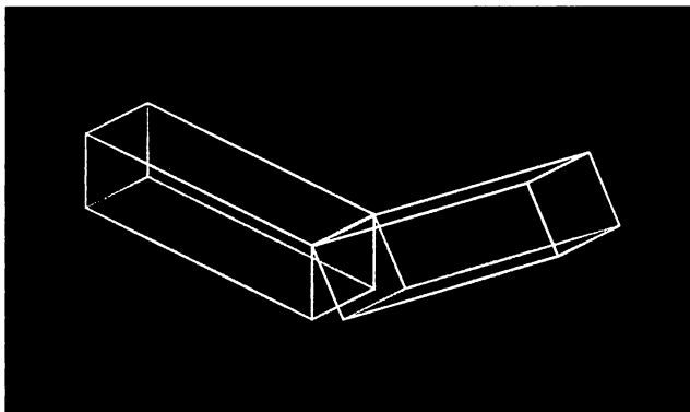
Figure 3-25 Robot Arm
