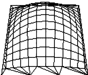
Figure 12-4 NURBS Surface
