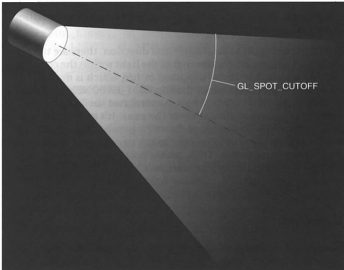
Figure 5-2 GL_SPOT_CUTOFF Parameter
