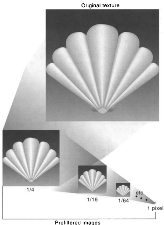
Figure 9-6 Mipmaps
