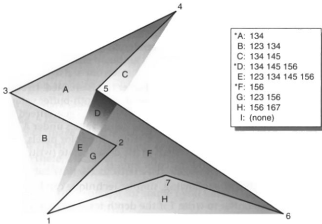
Figure 14-2 Concave Polygon
