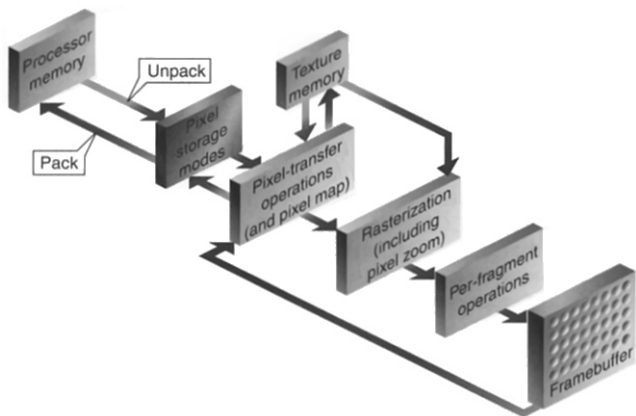
Figure 8-5 Imaging Pipeline
