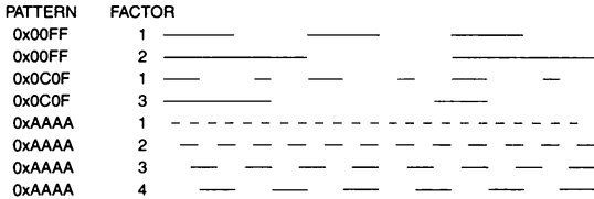
Figure 2-8 Stippled Lines
