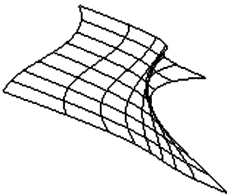
Figure 12-2 Bézier Surface
