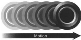
Figure 10-2 Motion-Blurred Object
