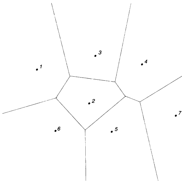
Figure 14-3 Dirichlet Domains
