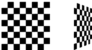
Figure 9-2 Texture-Mapped Squares
