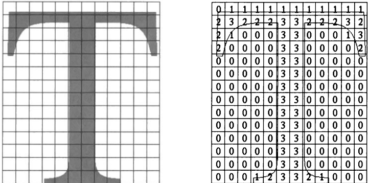
Figure 14-1 Antialiased Characters
