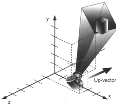
Figure 3-12 Using gluLookAt()
