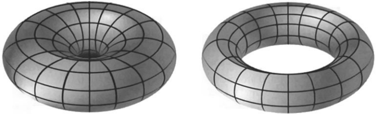
Figure 9-9 Texture-Map Distortion
