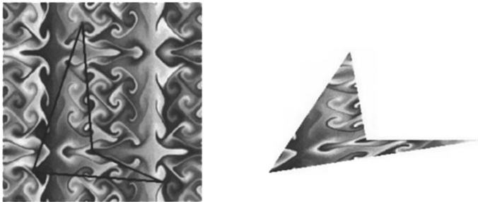
Figure 9-1 Texture-Mapping Process
