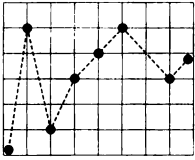
Figure 3-16 Viewport Rectangle
